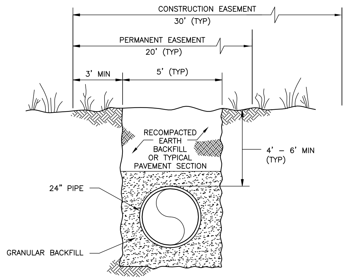
TYPICAL TRENCH AND EASEMENTS SECTION
