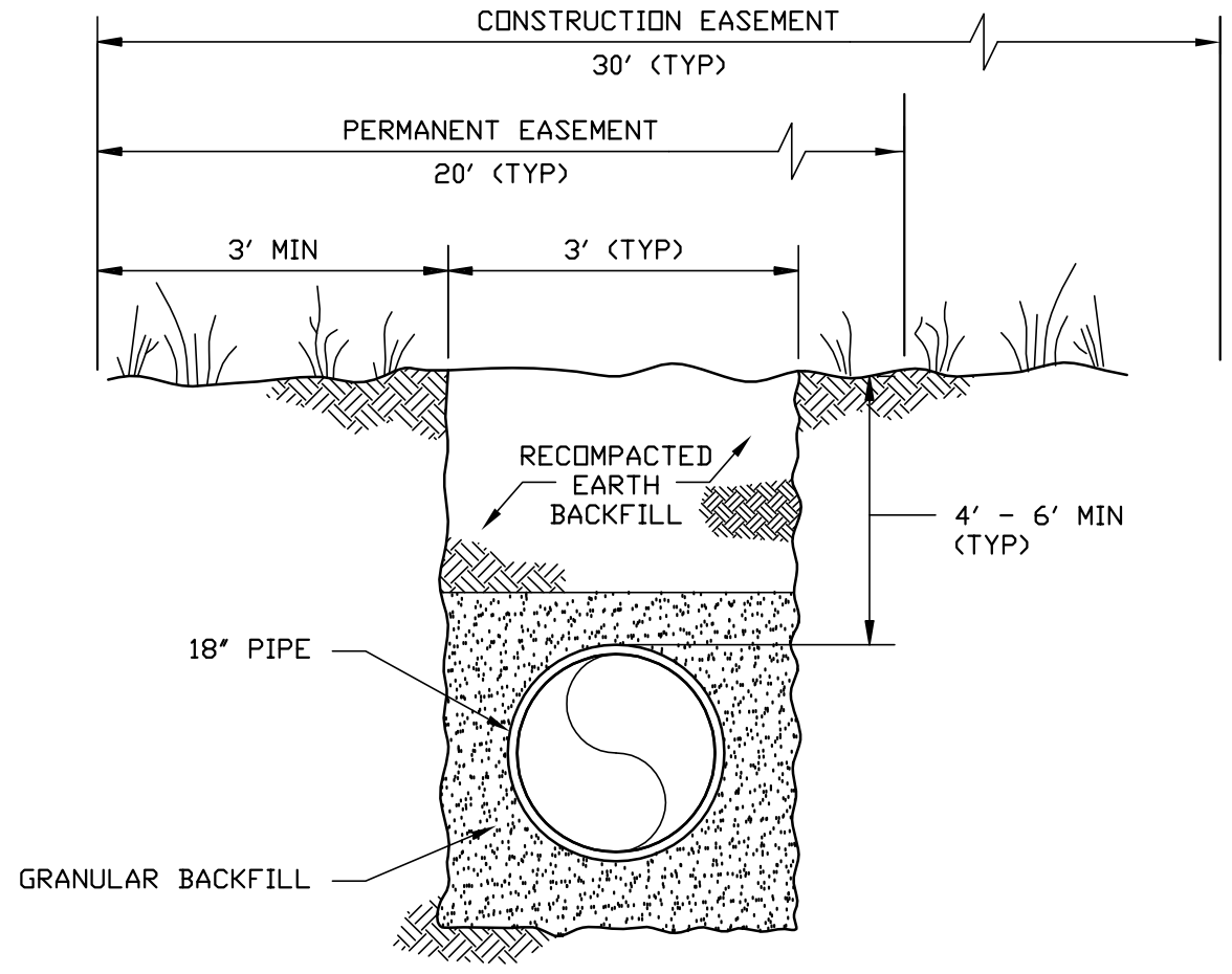
TYPICAL TRENCH AND EASEMENTS SECTION
